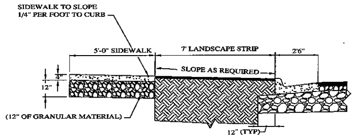
SIDEWALK CROSS-SECTION
